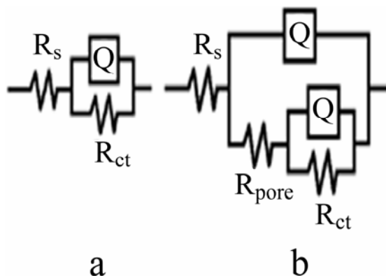
Fig. 8. a) equivalent circuit to fit the electrochemical impedance data of the titanium substrate and b) equivalent circuit to fit the electrochemical impedance data of the coated substrate
